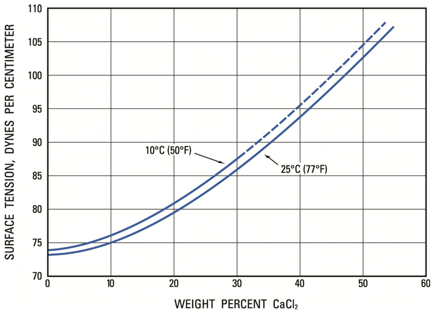
Figure 6: Surface Tension of Pure CaCl 2 Solutions
